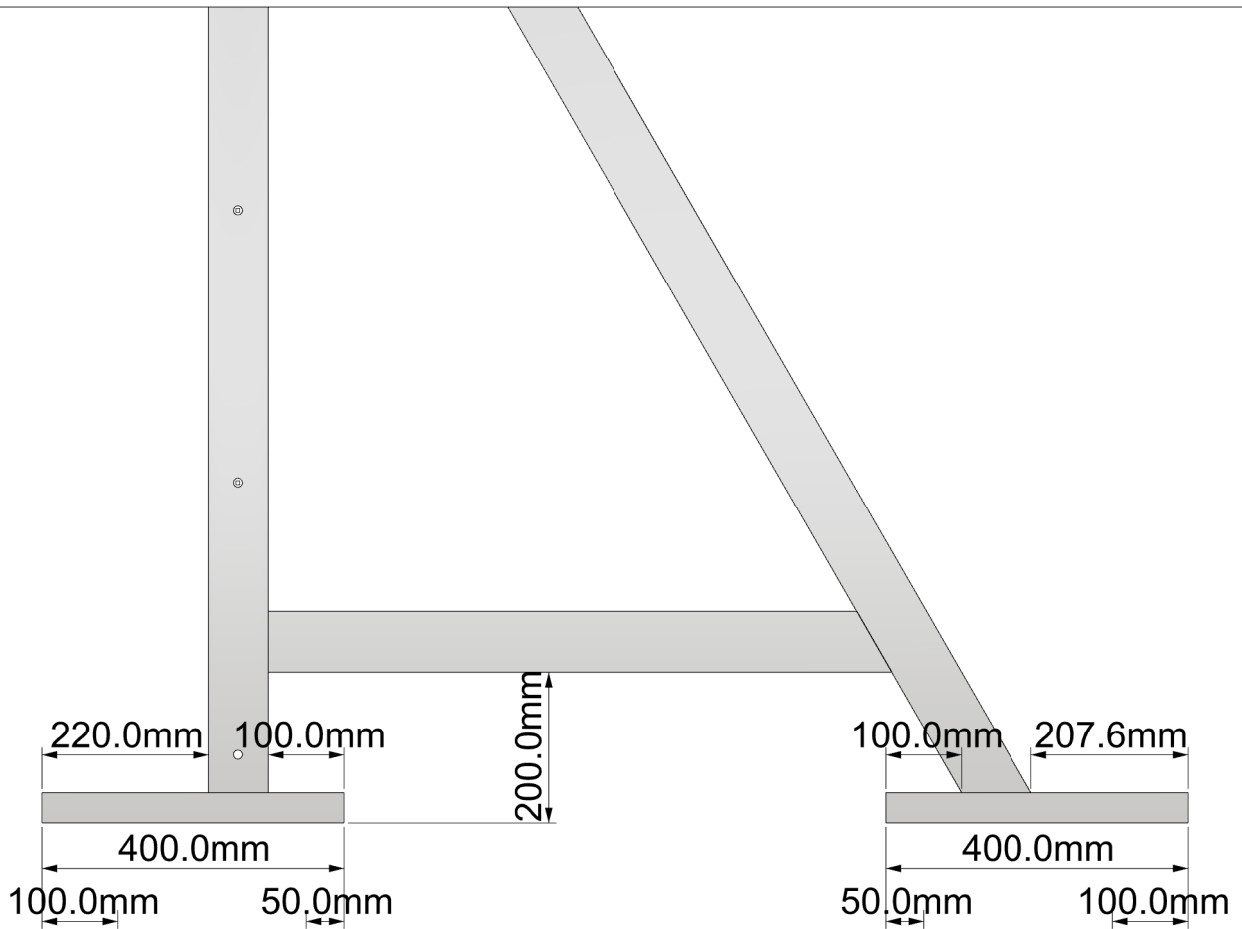
Plan Support A 1:10
