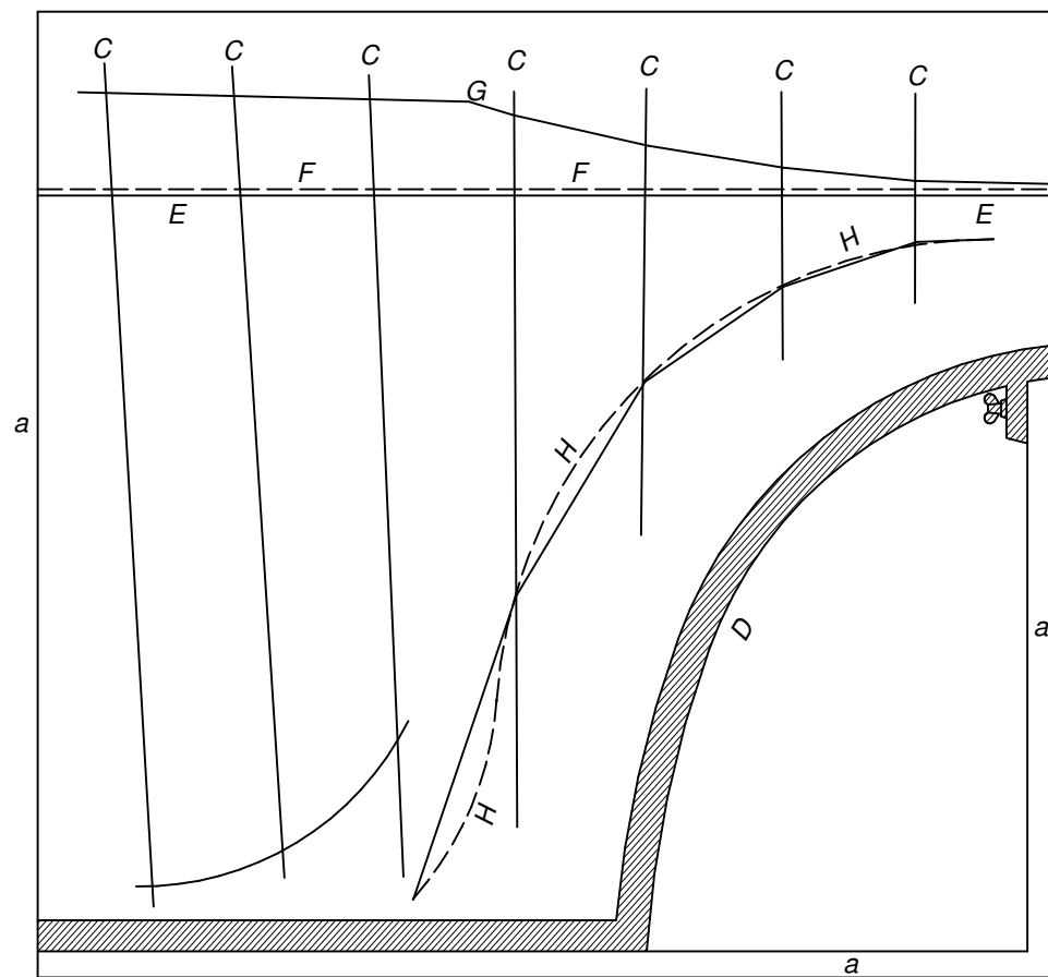
FIG. 1 PLAN OF BRIDGES.
