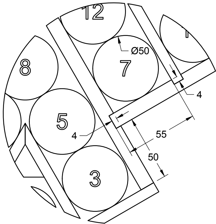
DETAIL A SCALE 1:1.75
