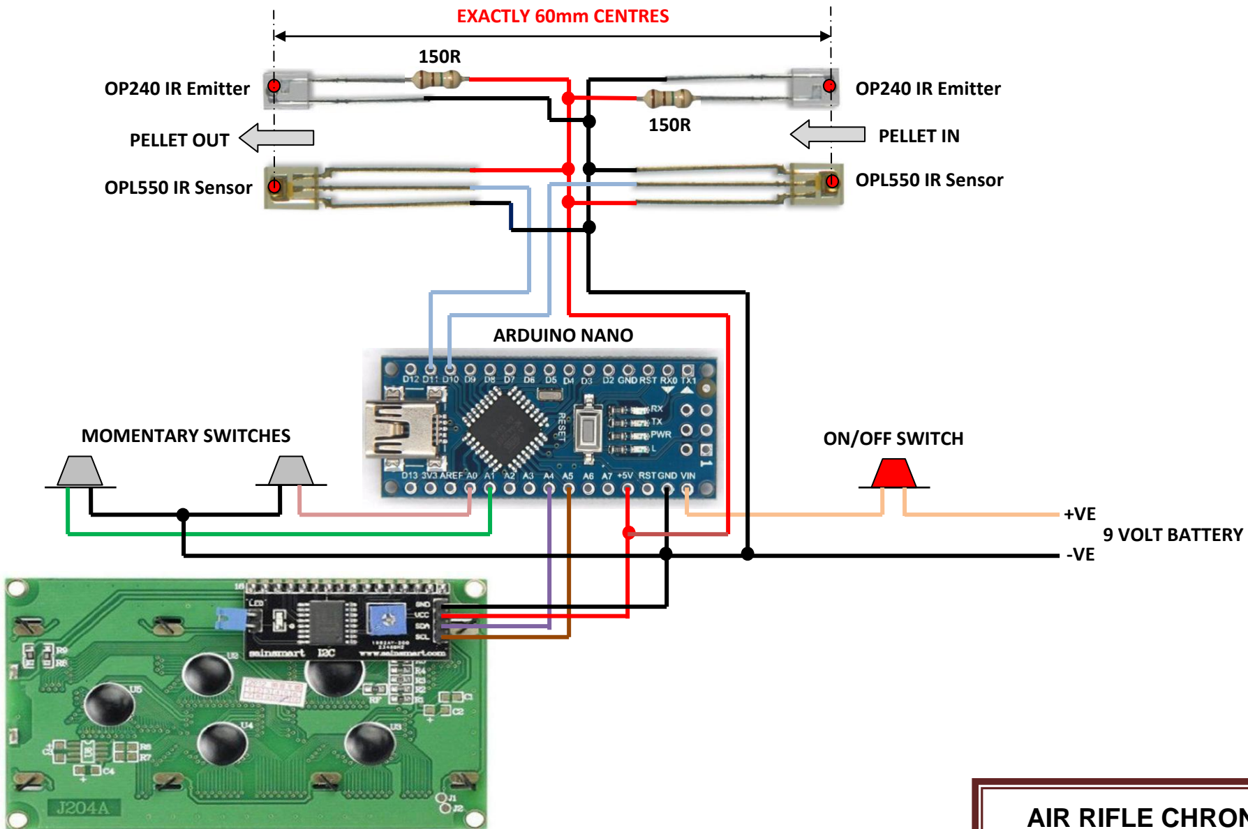
20X4 CHARACTER LCD 2004 with i2C SERIAL INTERFACE
