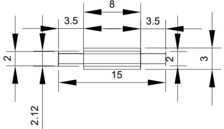
Moon32TDoubleGearAxle
