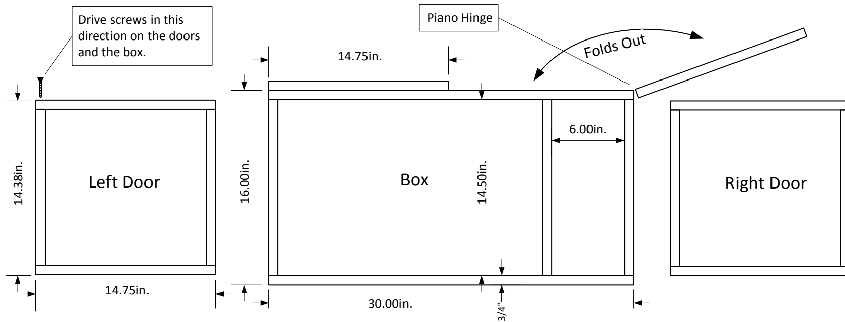
FRONT VIEW
