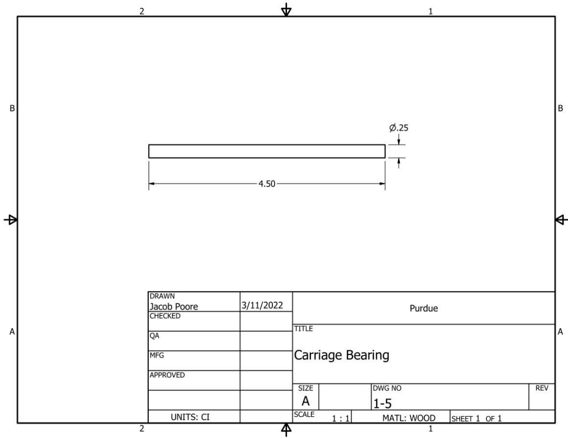
Fig. 6. Technical drawing of carriage bearing
