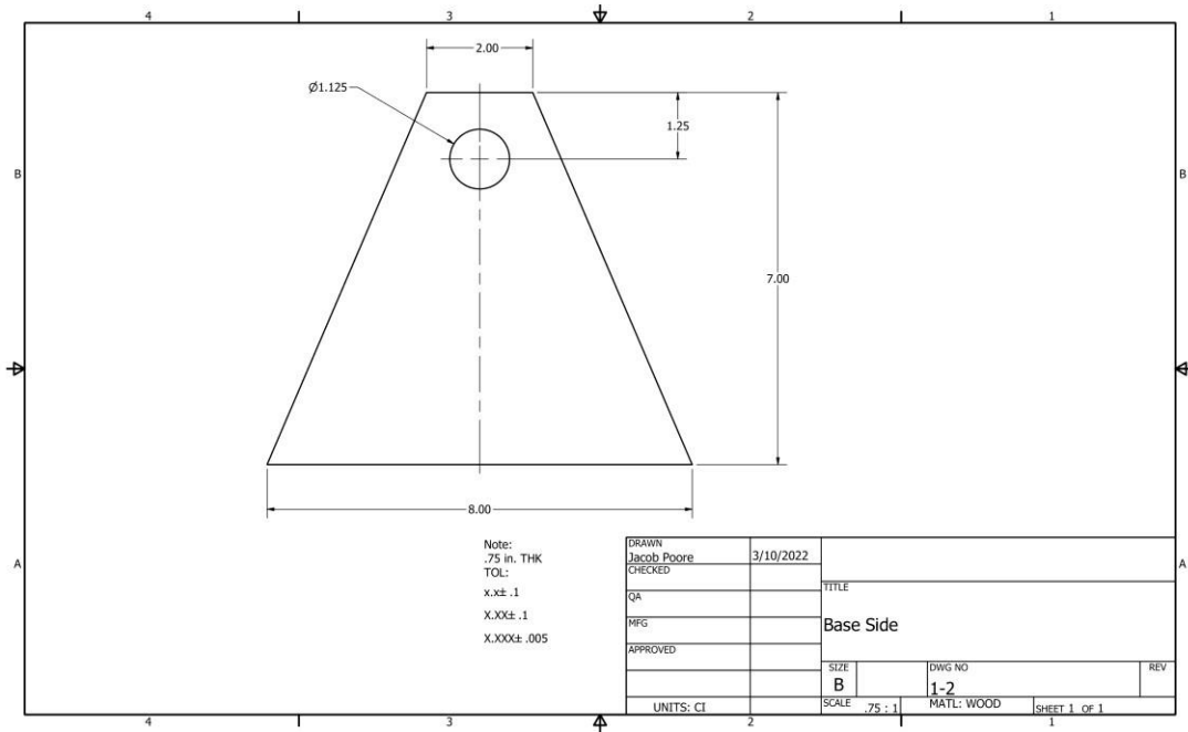
Fig. 3. Technical drawing of Ferris wheel base
