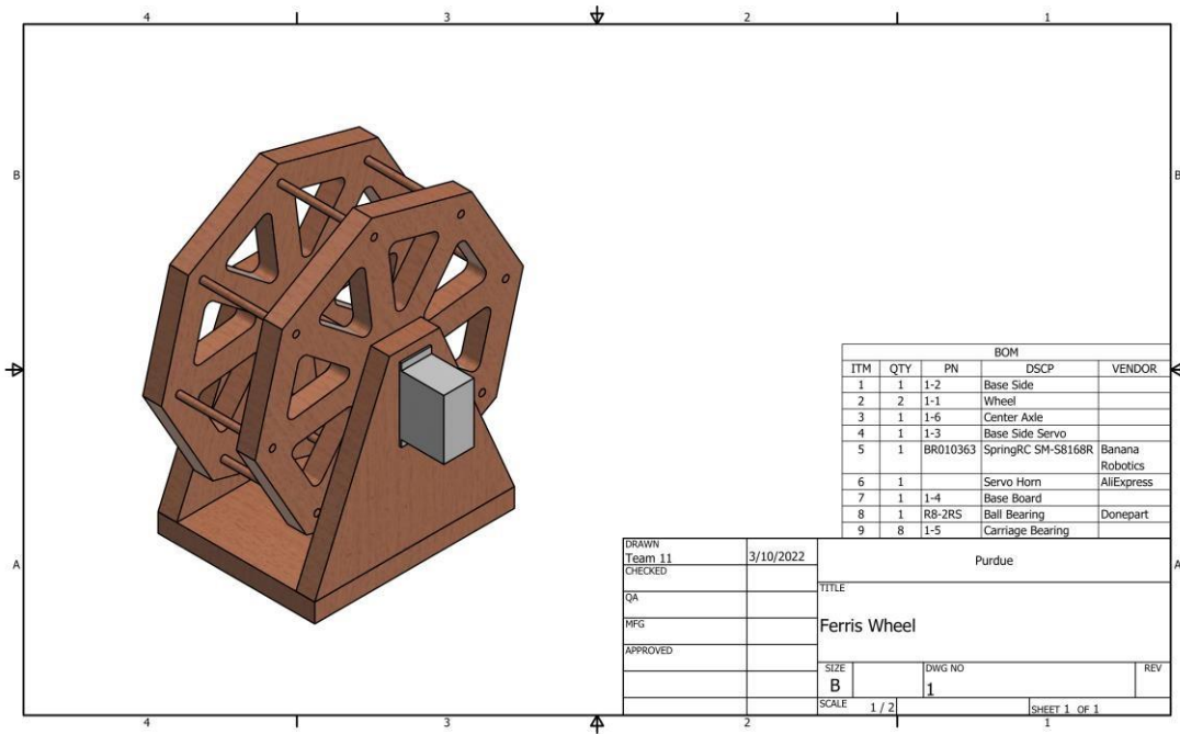
Fig.1. Three-dimensional view of assembled Ferris wheel model
