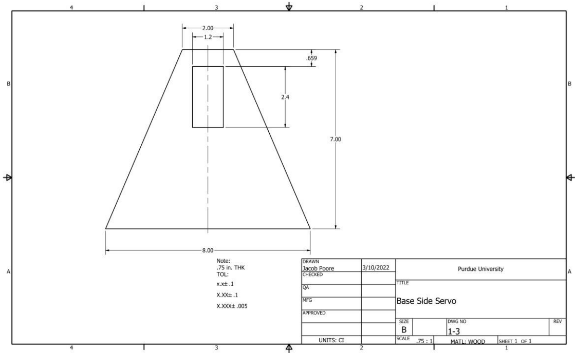
Fig. 5. Technical drawing of servo mount in the wheel's base
