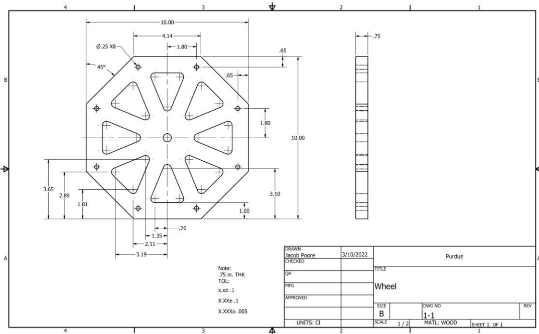
Fig. 4. Technical drawing of wheel section, side-on
