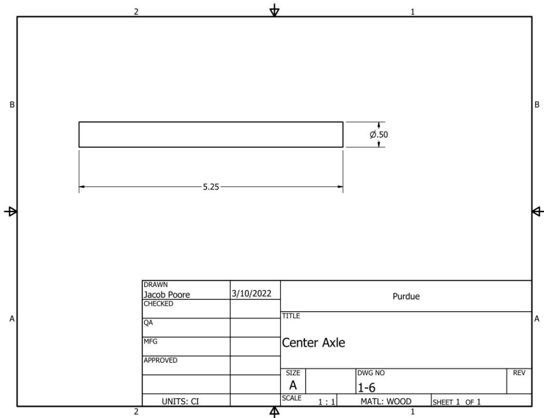
Fig. 8. Technical drawing of center axle
