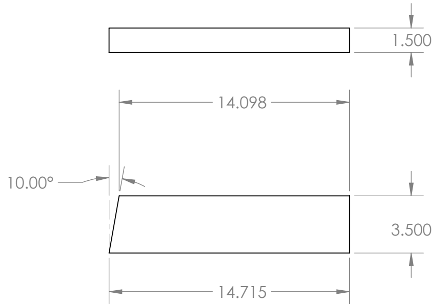
2X4 SIDE SEAT
