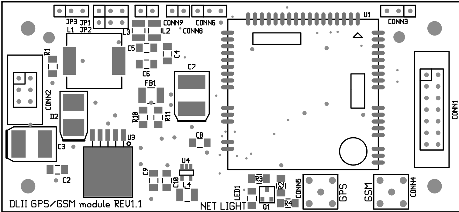
Pict.1 GPS/GSM Module, component layout, top side
