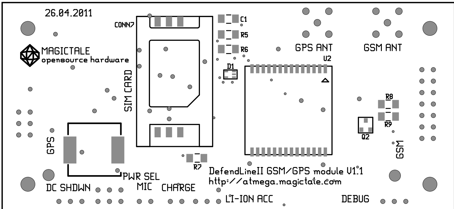
Pict.2 GPS/GSM Module, component layout, bottom side
