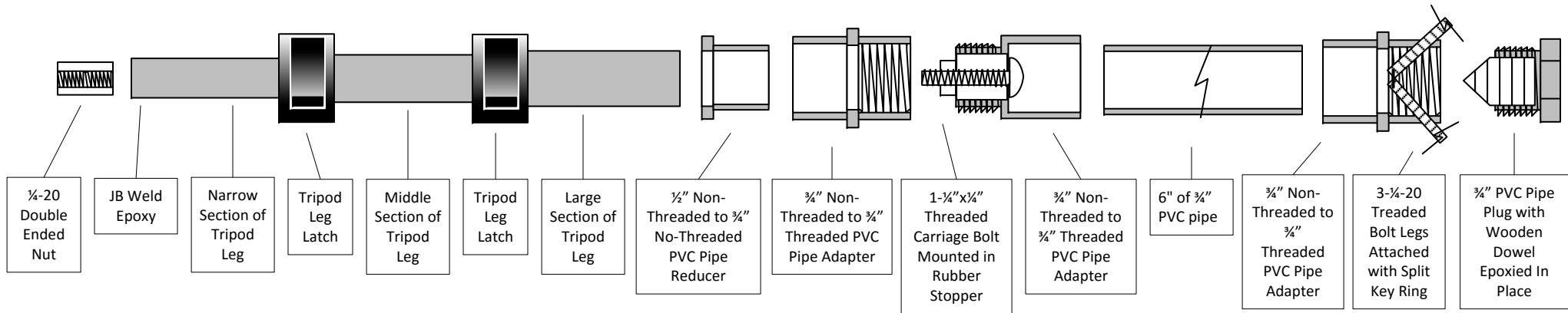
Exploded View
