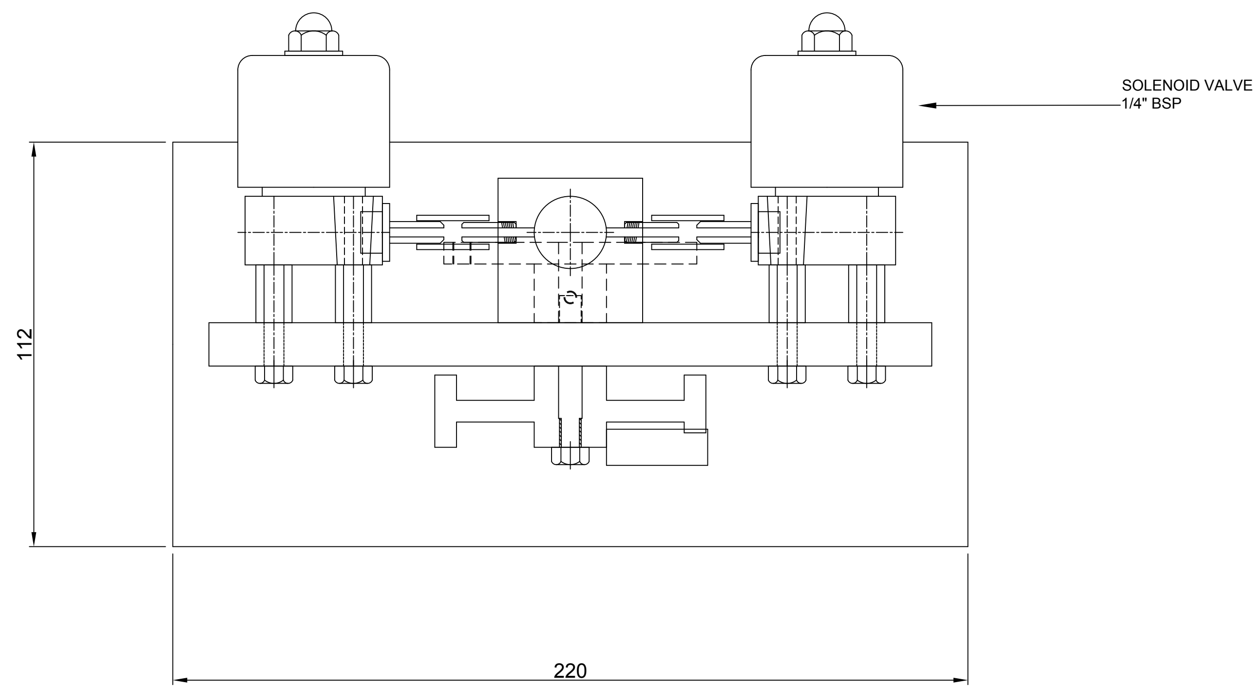
PLAN VIEW
