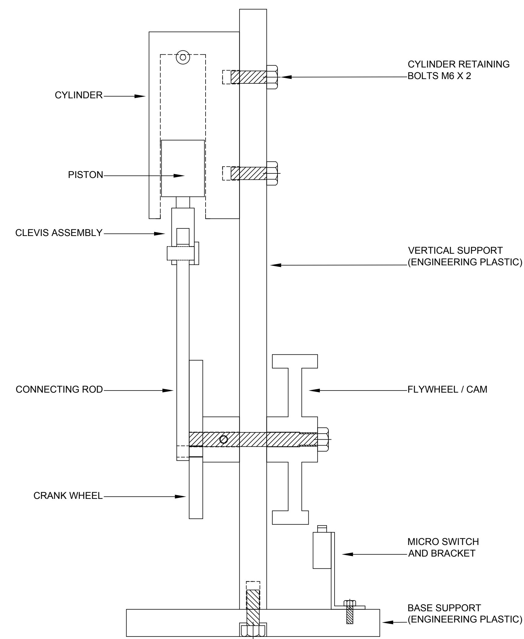
SECTIONAL VIEW
