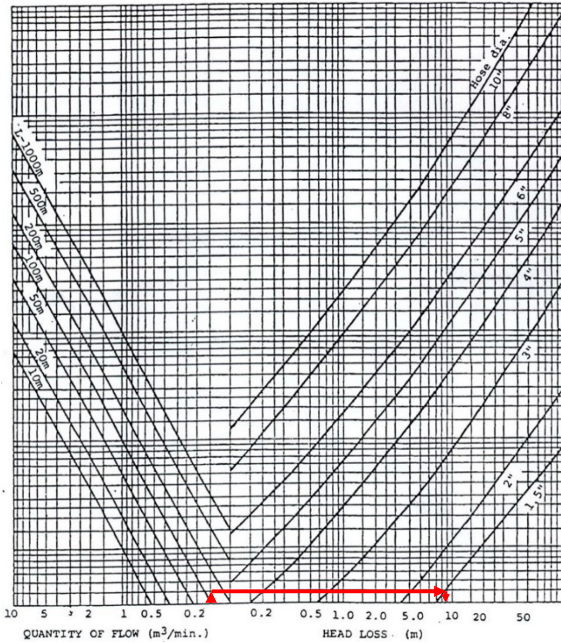
Layflat Hose Friction from National Pump and Energy Website
