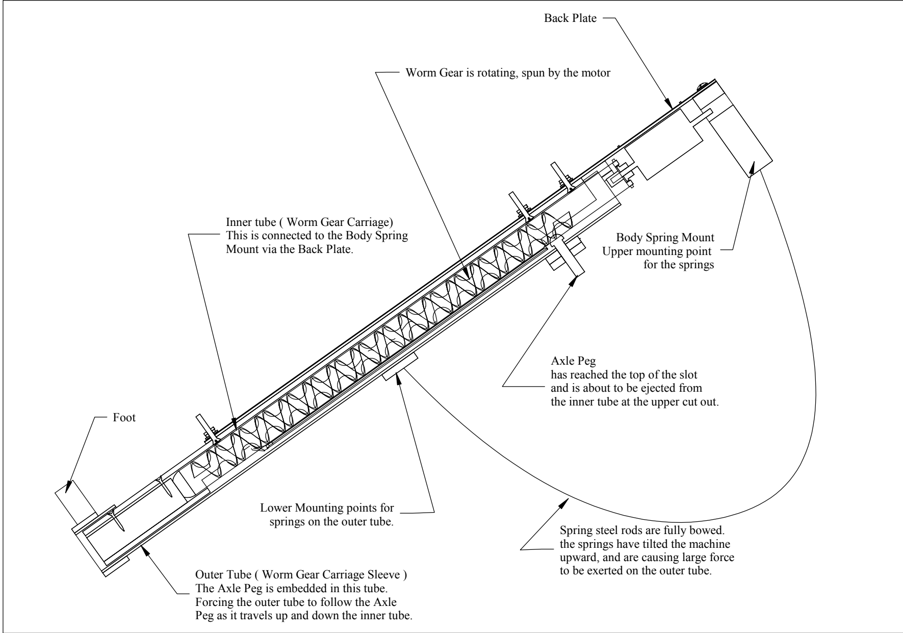
Operation - Fully Compressed Cross section view
