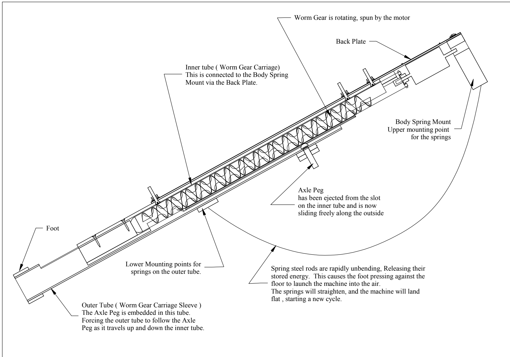
Operation - Leaping Cross section view
