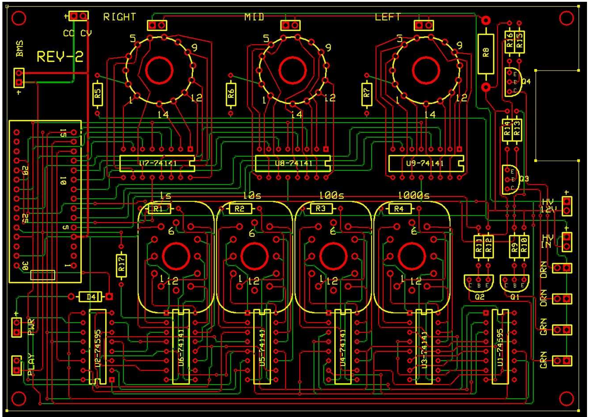
PCB Layout
