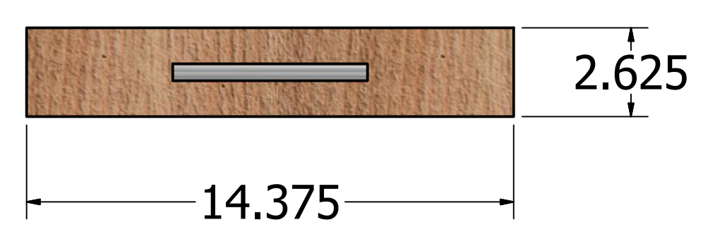
Drawer for 14.5" Wide x 2.75" High x 17.75" Deep Opening (Same Construction for Remaining Drawers)
