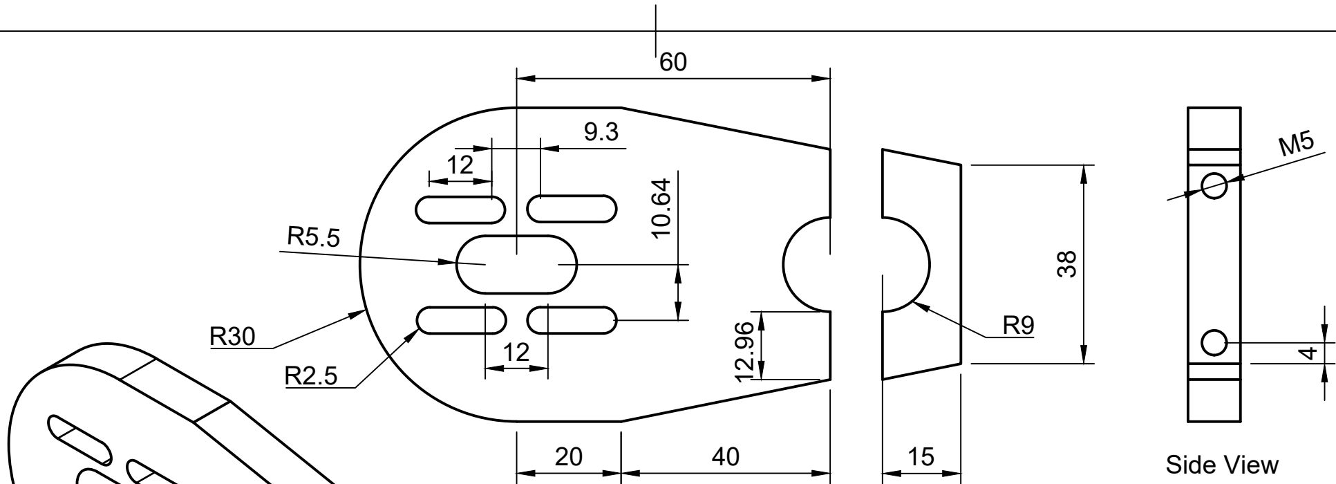
Front View
