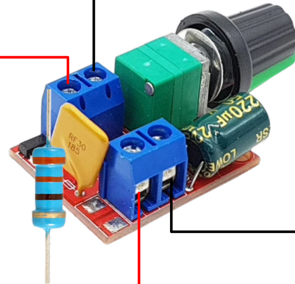
Speed Controller
