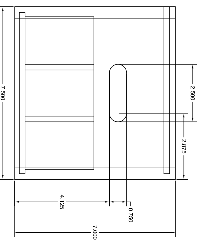
Detail for Lid Finger Groove
