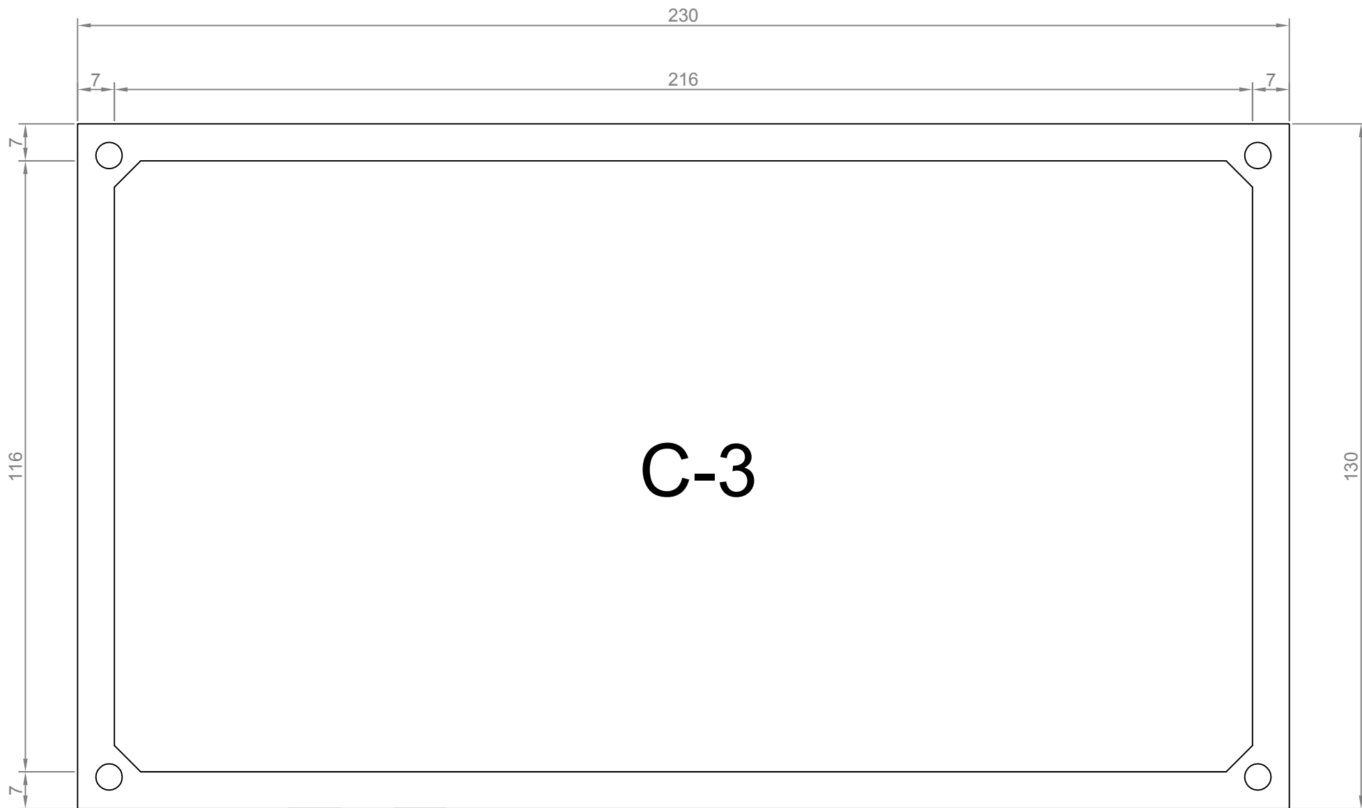
Shipping Container Tissue Box by ardeepapercraft (all size in mm)
