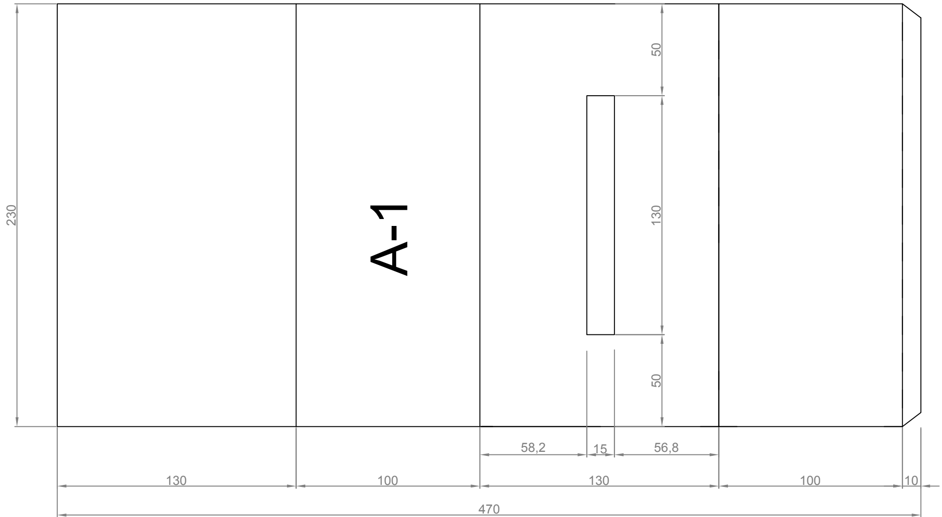
Shipping Container Tissue Box by ardeepapercraft (all size in mm) Note: size not to scale
