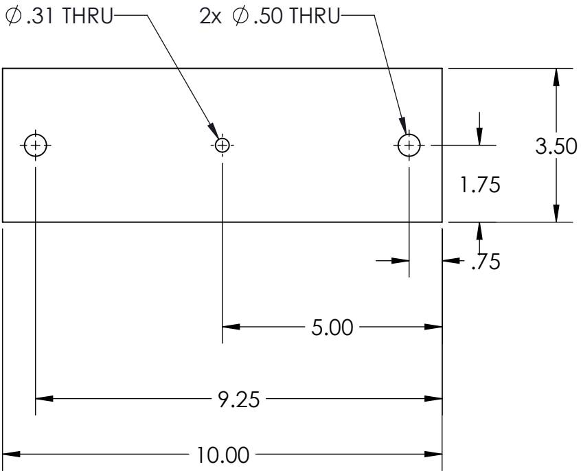
TESTRBOT TOP CROSS BEAM VERSION 1.0
