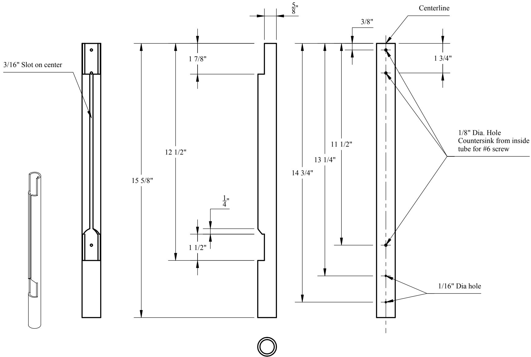
Worm Gear Carriage Body Detail material : 3/4" Schedule 40 PVC pipe
