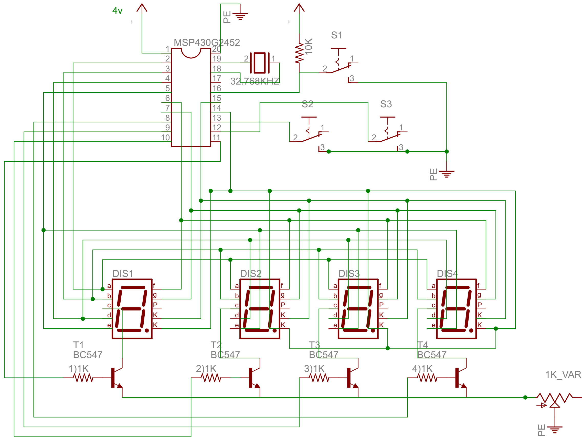
Digital Clock - using MSP430G2452
