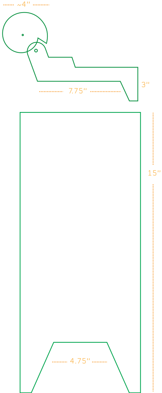
Foot Tap Amplifier Side View (2 Sides) Cam and Hammer Arm - Side View
