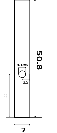
Top/Bottom View
