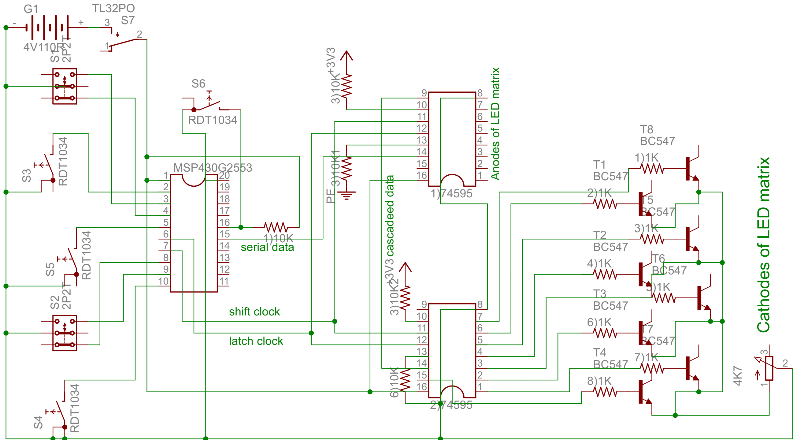
Gameboy Schematic Diagram
