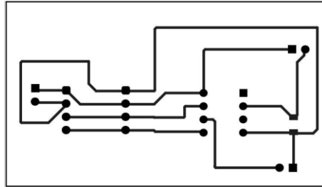
KY-013 Analog Temperature Sensor
