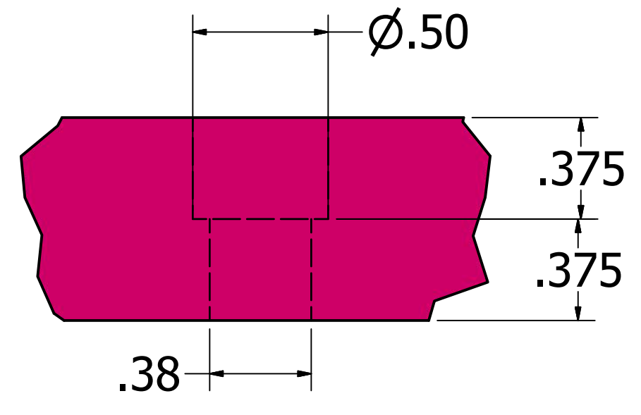
DETAIL D SCALE 2
