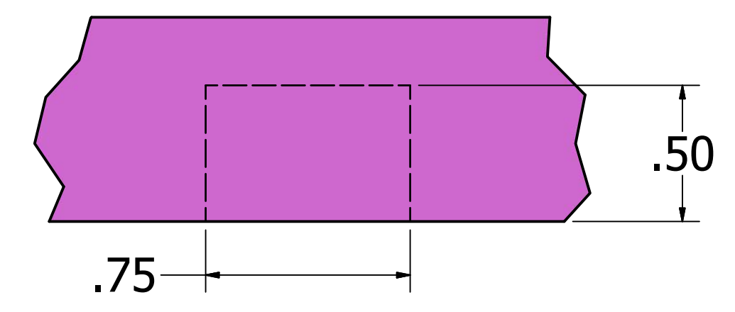
DETAIL E SCALE 2
