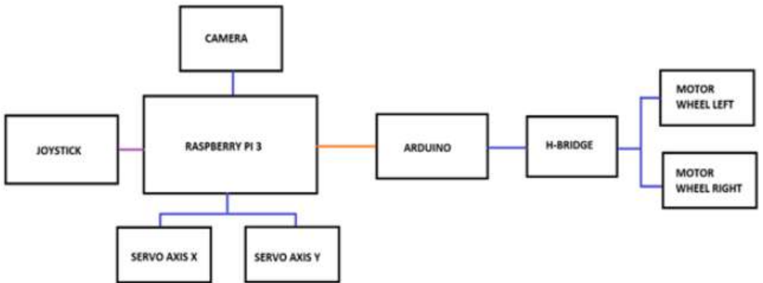
Photo x: Simple electric schemes.
